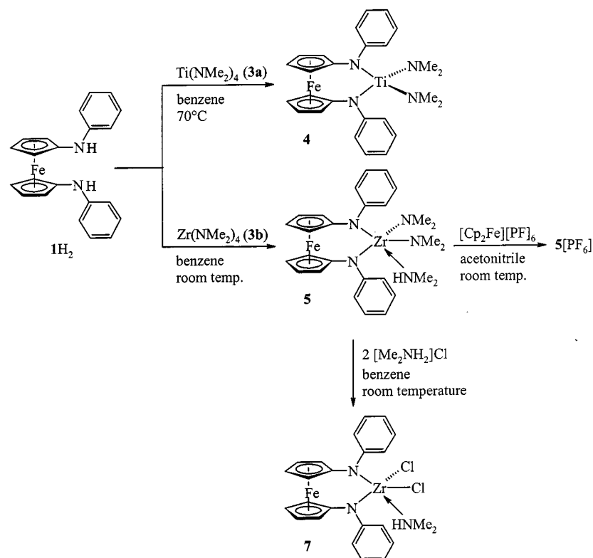
Scheme 1. Synthesis of the chelate complexes 4 , 5 , 5 [PF 6 ], and 7
