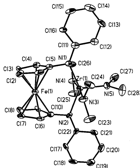
Figure 1. Molecular structure of 5 in the crystal; selected bond lengths (pm) and angles (°): Zr(1)–N(1) 212.8(7), Zr(1)–N(2) 215.3(7), Zr(1)–N(4) 215.4(7), Zr(1)–N(5) 205.7(7), N(1)–C(5) 142.3(11), N(1)–C(11) 139.5(10), N(2)–C(10) 141.3(10), N(2)–C(22) 138.9(9); N(3)–Zr(1)–N(5) 92.5(3), N(4)–Zr(1)–N(5) 96.0(3)
