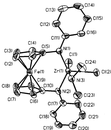
Figure 2. Molecular structure of 7 in the crystal; selected bond lengths (pm) and angles ( ^{\circ} ): Zr(1)–N(1) 206.0(4), Zr(1)–N(2) 207.6(4), Zr(1)–N(3) 238.3(4), Zr(1)–Cl(1) 245.95(16), Zr(1)–Cl(2) 241.76(14), N(1)–C(5) 141.6(6), N(1)–C(11) 141.4(6), N(2)–C(10) 141.9(6), N(2)–C(17) 139.4(6); N(3)–Zr(1)–Cl(2) 81.56(10), Cl(1)–Zr(1)–Cl(2) 91.02(5)
